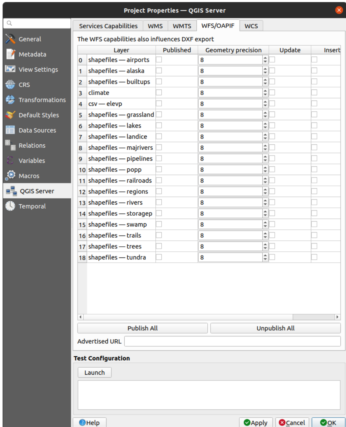
Fig. 2.5: Definitioner i fliken WFS/OAPIF
